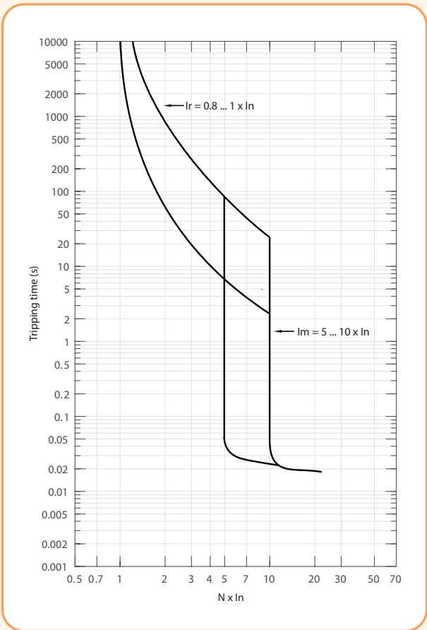
NBS-TMD 250/3 (200, 250A) I/t characteristic
