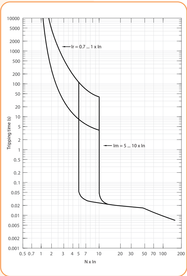
NBS-TMD 400/3 (315, 400A) I/t characteristic
