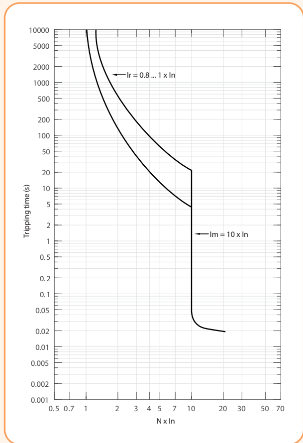
NBS-TMS 100/3 (50, 63A) I/t characteristic
