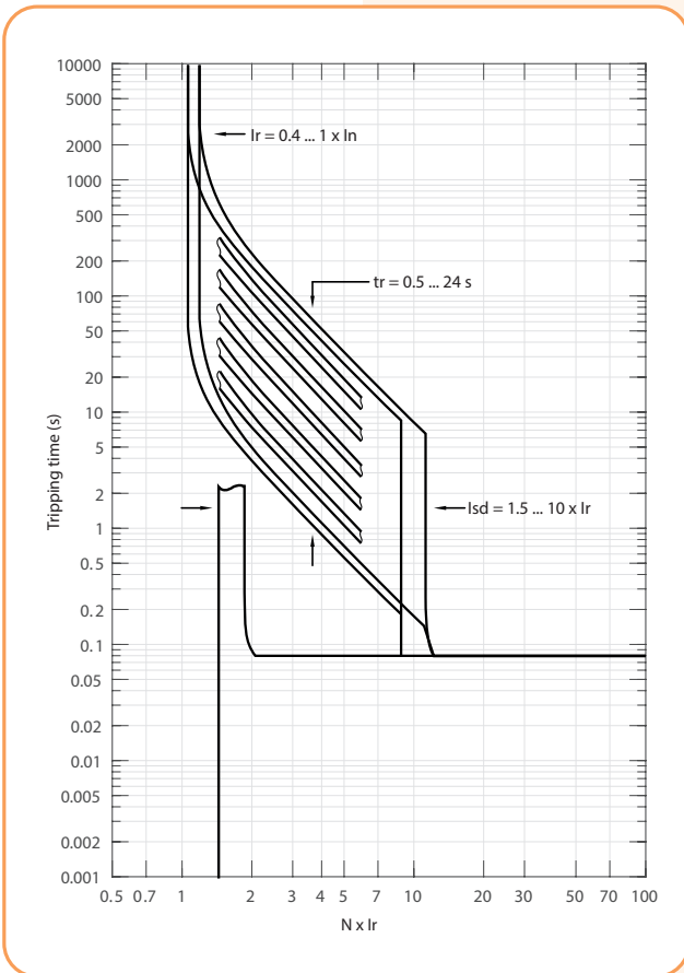
NBS-E (800 - 1600A) I/t characteristic
