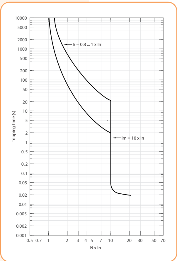
NBS-TMS 160/3 (125, 160A) I/t characteristic
