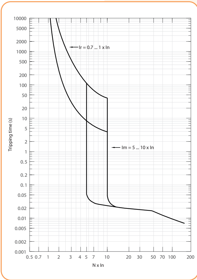
NBS-TMD 630/3 (500, 600A) I/t characteristic
