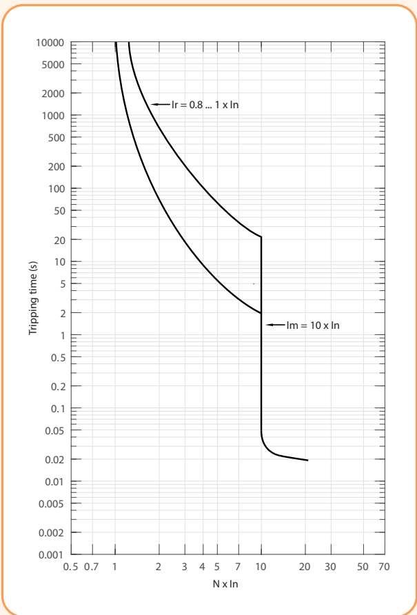
NBS-TMS 100/3 (80, 100A) I/t characteristic
